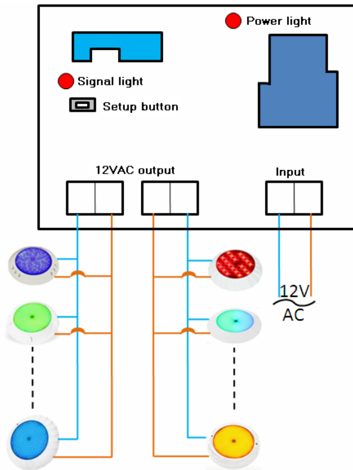
Fig2 wiring of RC01
